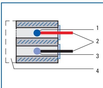
1 = Katalysatorpellistor 2 = Elektroanschlüsse 3 = Interpellistor 4 = Diffusionssieb
